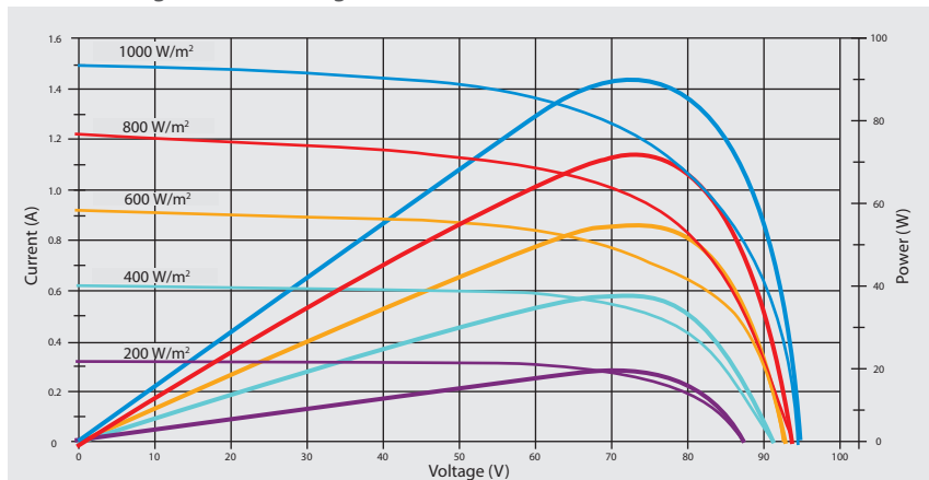
Current-Voltage & Power-Voltage Curve (90 W)
