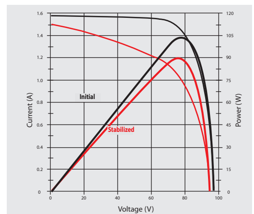
I-V Curve comparison between Stabilized and Initial (90 W)
